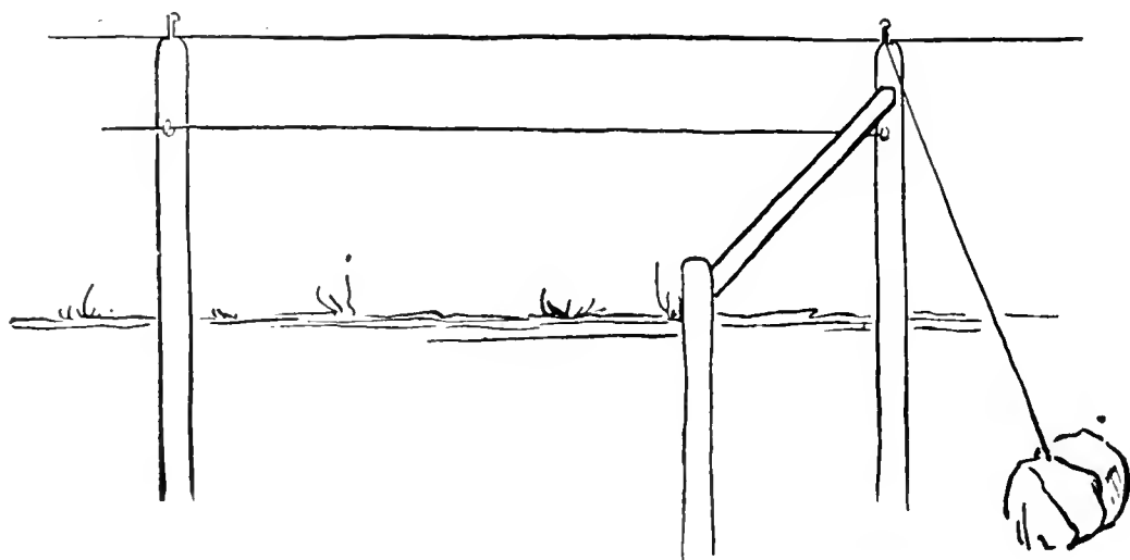
Fig. 66—Method of Bracing the End Posts
